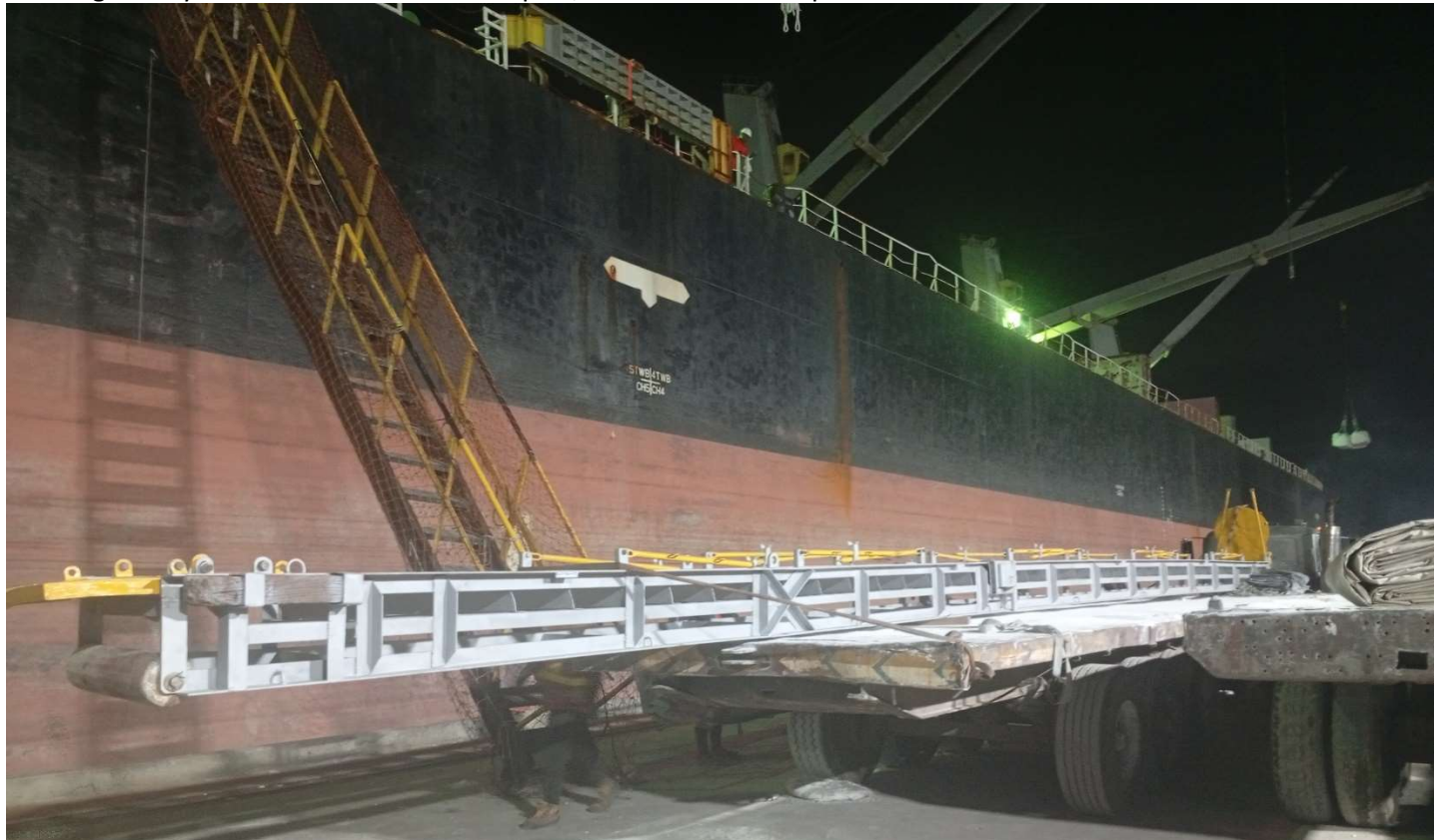
Trucking of fully refurbished ladder back to port, to load back on Ship
