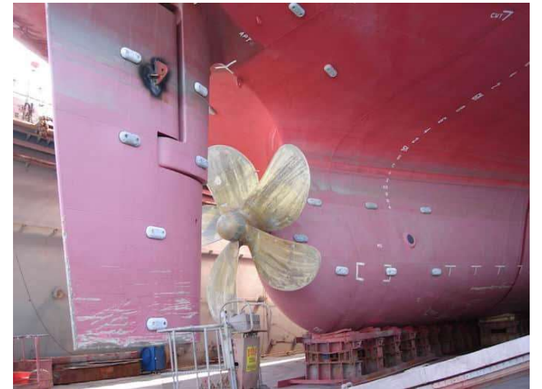
Rudder Repairs in Floating dock
